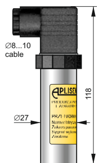
PD type PD316 type IP65
