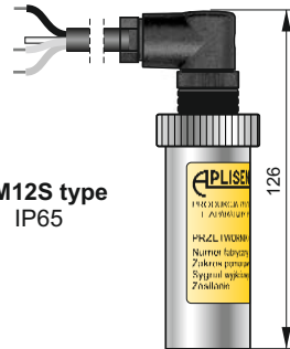
PM12SK type IP67
