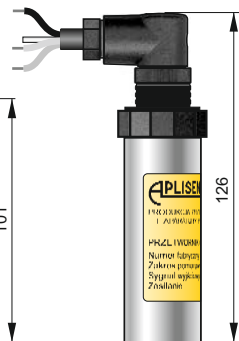
PM12K type IP67
